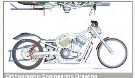
Orthographic Engineering Drawing
